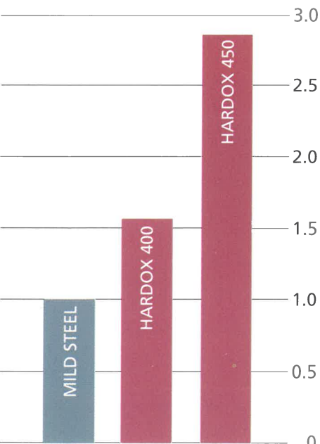
Relative useful life. Comparison between mild steel (150 HBW), HARDOX 400 and HARDOX 450.
